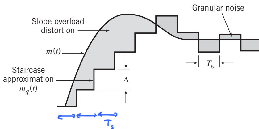
Figure 73: Two different forms of error in DM
