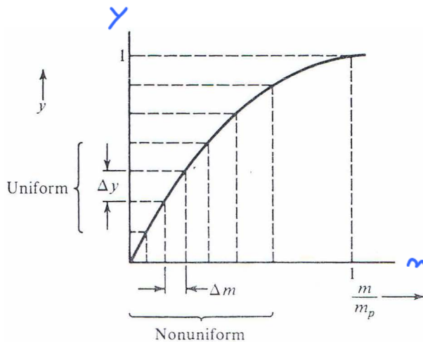
Figure 70: An example of a compressor characteristic curve [6, Fig 6.15b p. 326]
