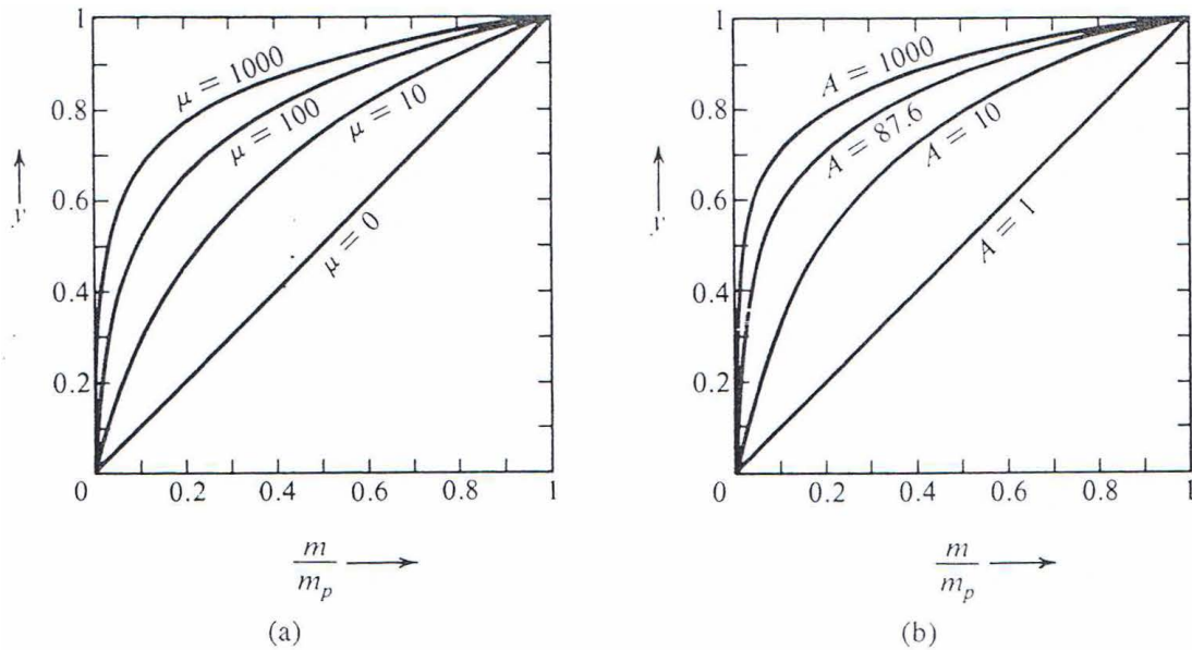
Figure 71: (a) \mu -law characteristic. (b) A -law characteristic. [6, Fig 6.16 p. 326]
