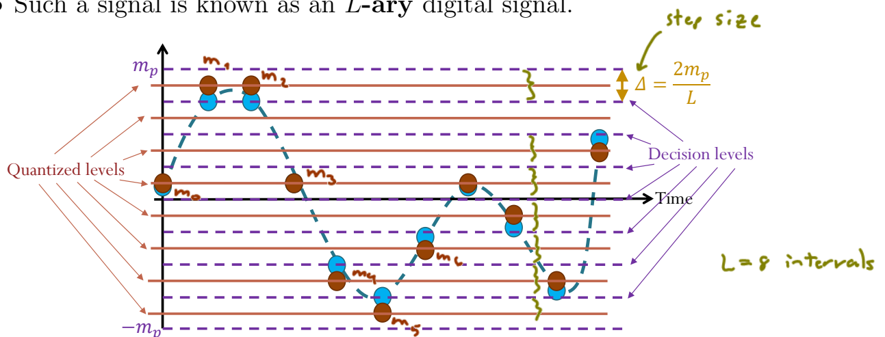
Figure 66: Quantized levels
